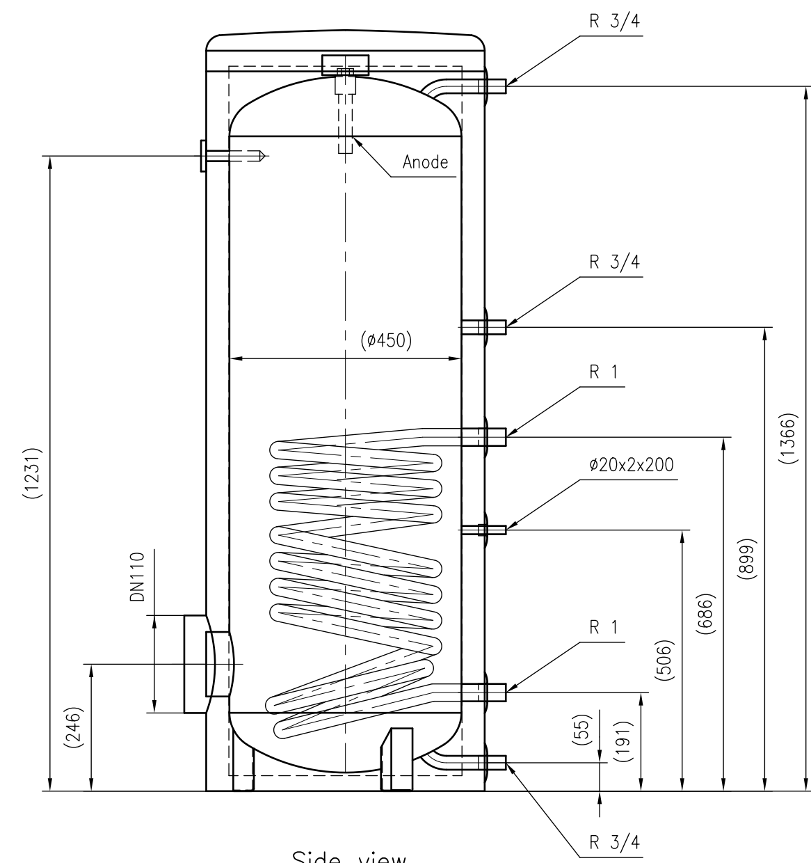
Side view
